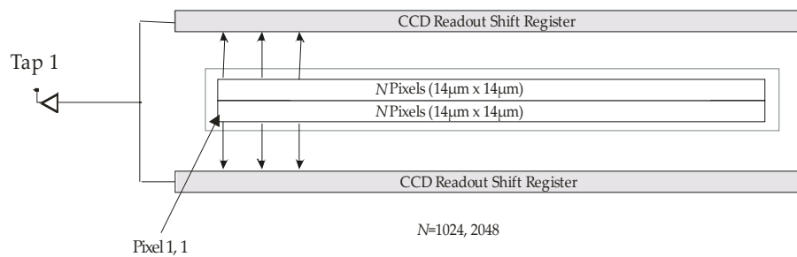
Figure 2: 1 Tap Sensor Block Diagram (SG-10-01K40, SG-10-02K40)
