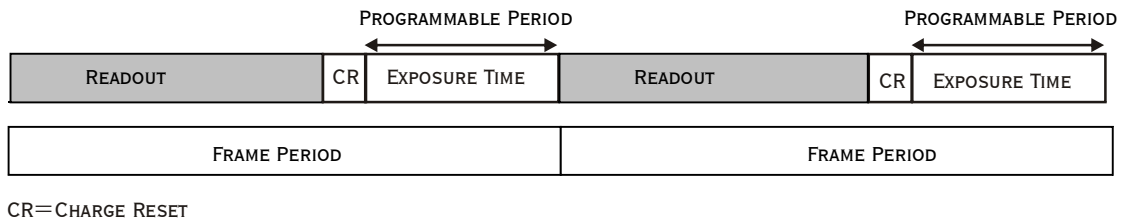
Figure 23: Mode 8 Timing
