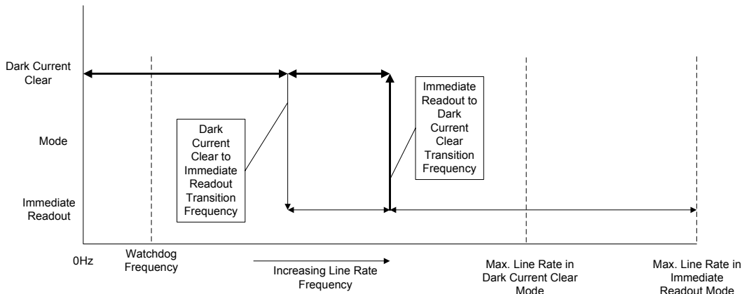
Figure 26: Gate Dark Current Clear
