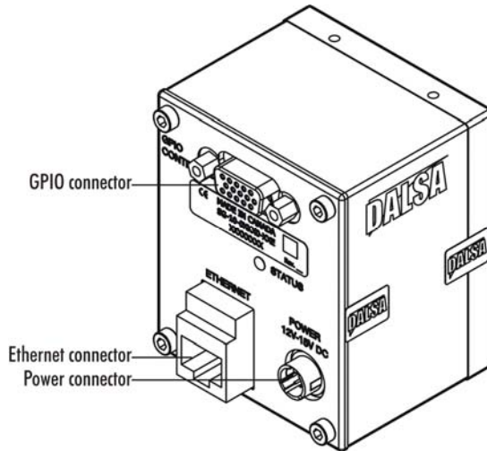
Figure 8: Spyder 3 GigE Input and Output Connectors
