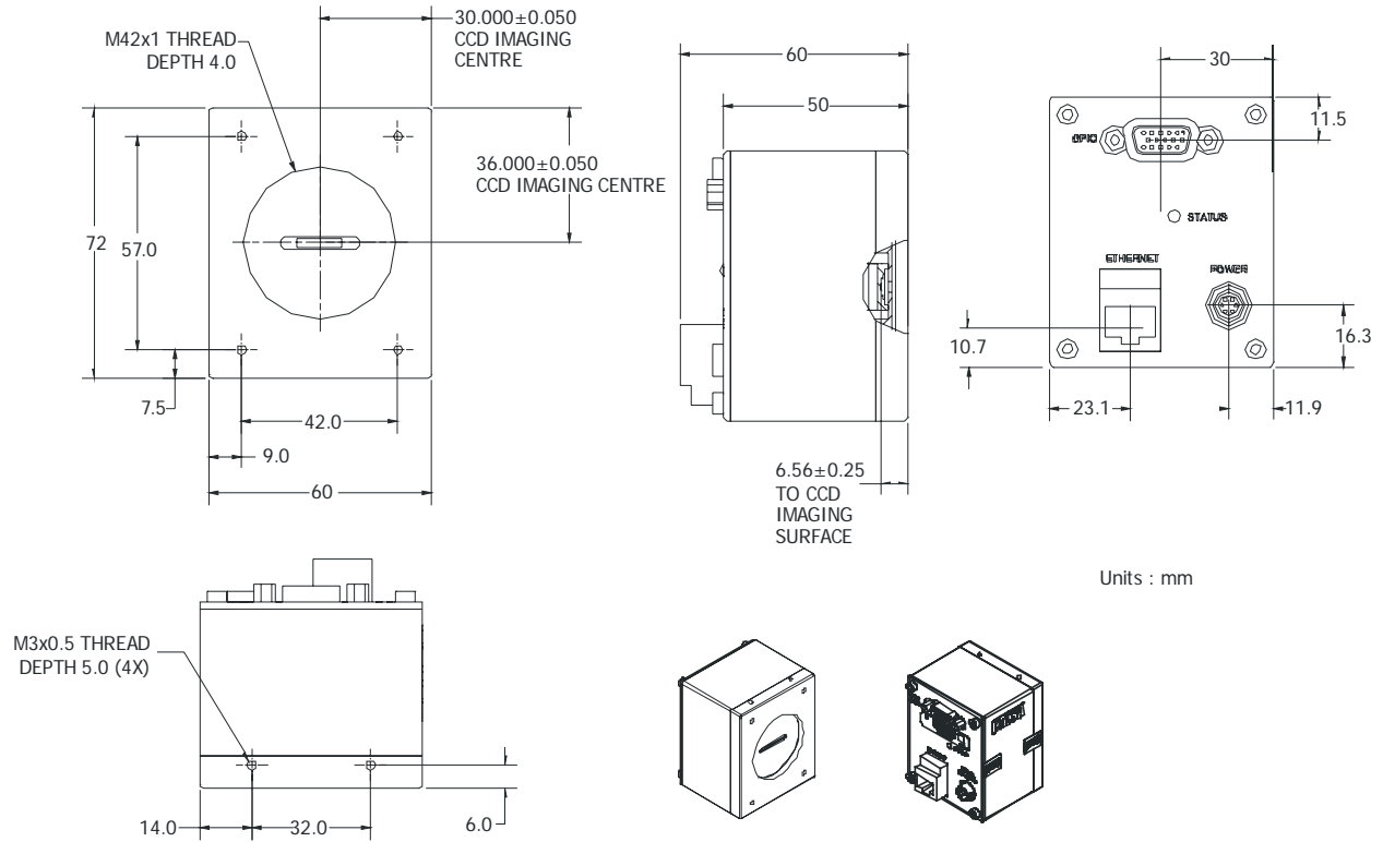
Figure 18: Spyder 3 GigE Heatsink Mechanical Dimensions
